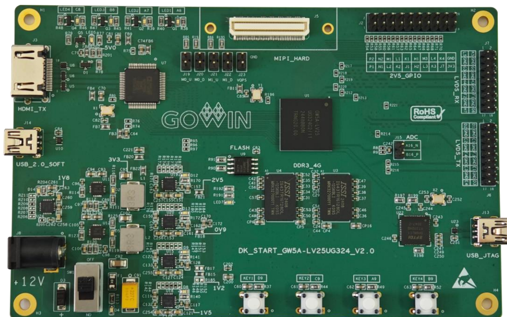
Figure 2-1 DK_START_GW5A-LV25UG324_V2.0 Development Board
