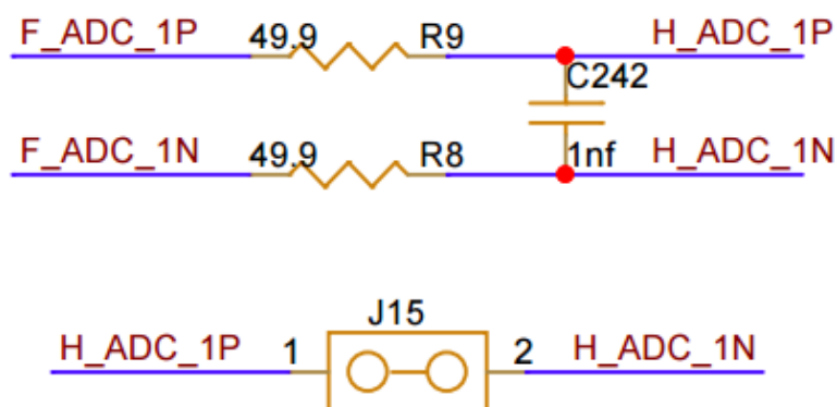
Figure 3-12 ADC Schematic
