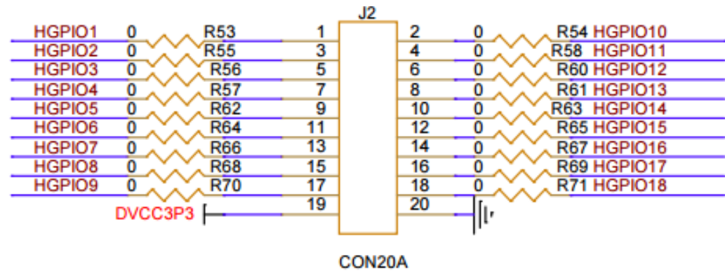
Figure 3-10 Schematic Connection Diagram of GPIO
