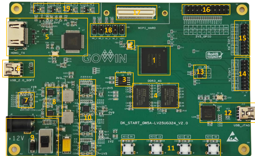
Figure 2-3 PCB Components
